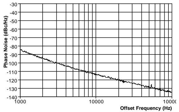
Figure 6 - Phase Noise at 650MHz
