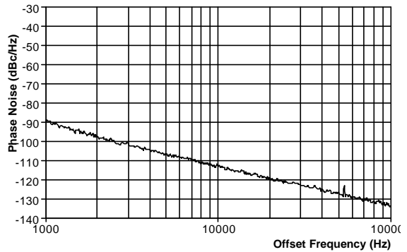
Figure 4 - Phase Noise at 450MHz
