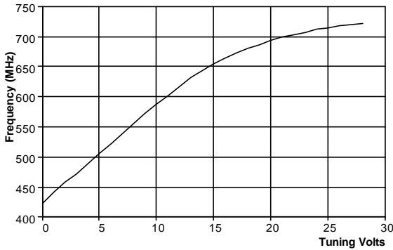
Figure 1 - Tuning Law
