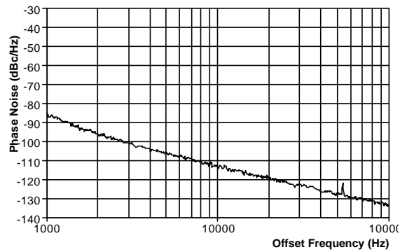
Figure 5 - Phase Noise at 550MHz
