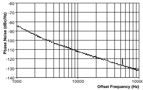
Figure 5 - Phase Noise at 800MHz
