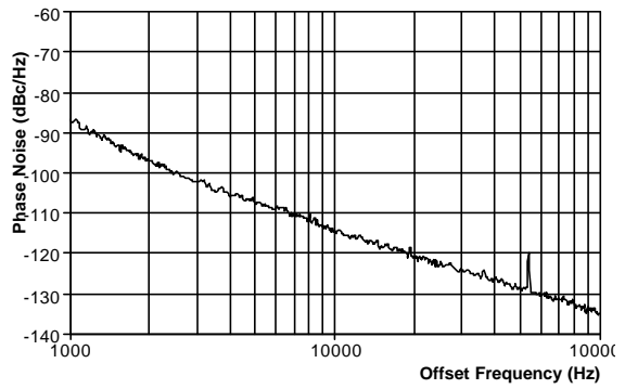
Figure 4 - Phase Noise at 700MHz
