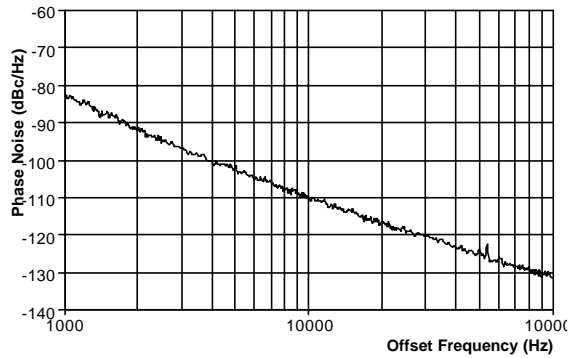
Figure 6 - Phase Noise at 900MHz
