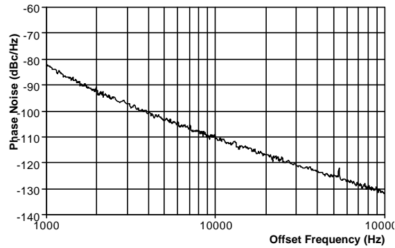
Figure 5 - Phase Noise at 850MHz
