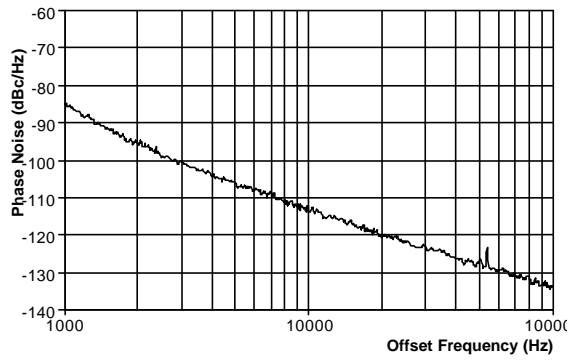
Figure 4 - Phase Noise at 750MHz
