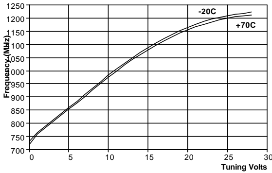
Figure 8 - Tuning Law over Temperature
