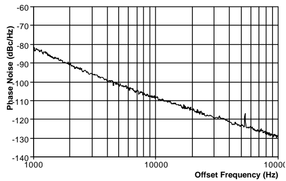
Figure 5 - Phase Noise at 900MHz
