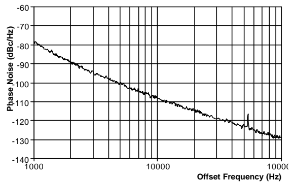
Figure 6 - Phase Noise at 1000MHz
