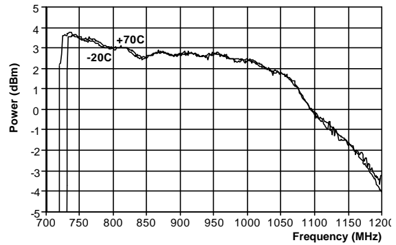
Figure 9 - Output Power over Temperature
