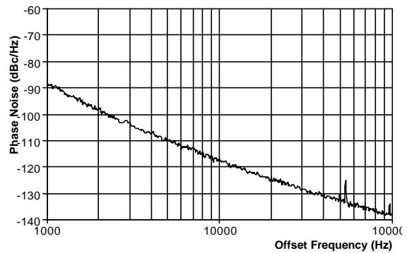
Figure 6 - Phase Noise at 550MHz
